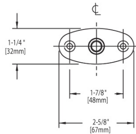
FLANGE DETAIL
